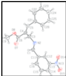
Fig. 1. The molecular structure of the title compound with the labeling scheme. Displacement ellipsoids are shown at the 40% probability level.
