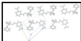
Fig. 2. Packing diagram of the title compound showing the formation of chains parallel to the [0\ 1\ \bar{1}] direction. Hydrogen bonds are shown as dashed lines.
